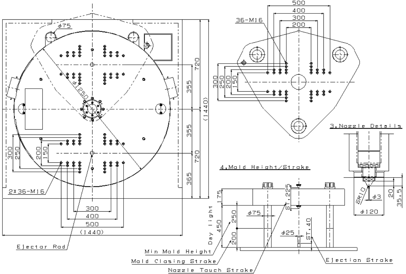
1. Rotary Table
